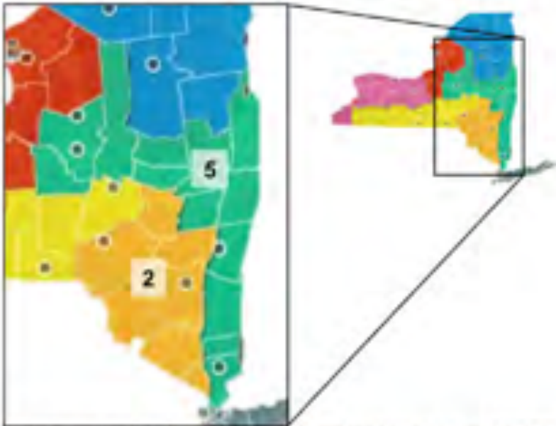
CIRAID climate regions 2 and 5, circles represent meteorological stations (NYSEIRDA).
